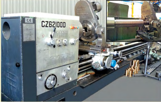
SONSUZ VİDA MAKİNASI / WORM SCREW MACHINE Ø 300 X 6000
